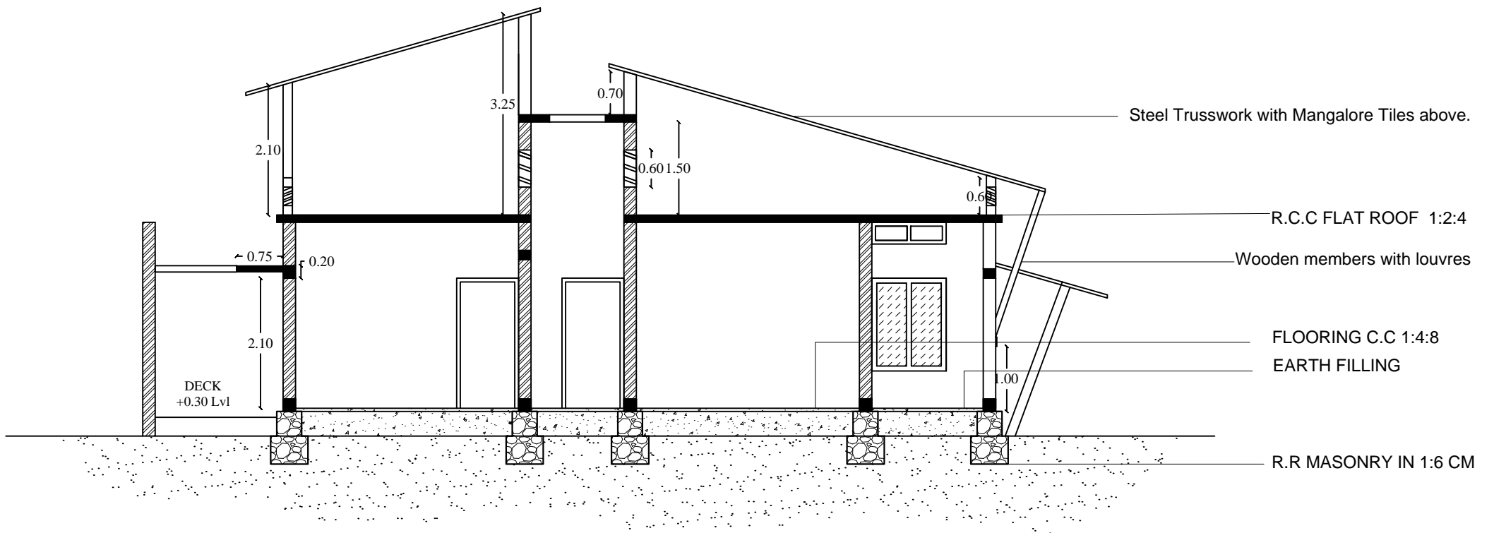
SECTION AA
