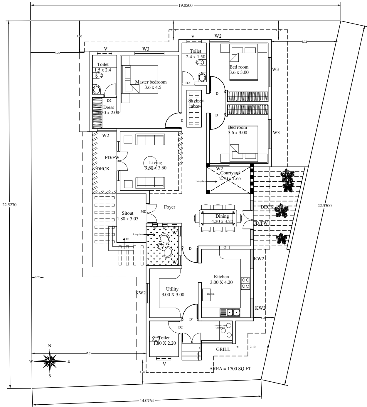
GROUND FLOOR PLAN WITH SITE
